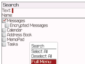
Figure 9. Short menu
