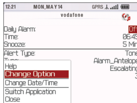
Figure 8. Full menu
